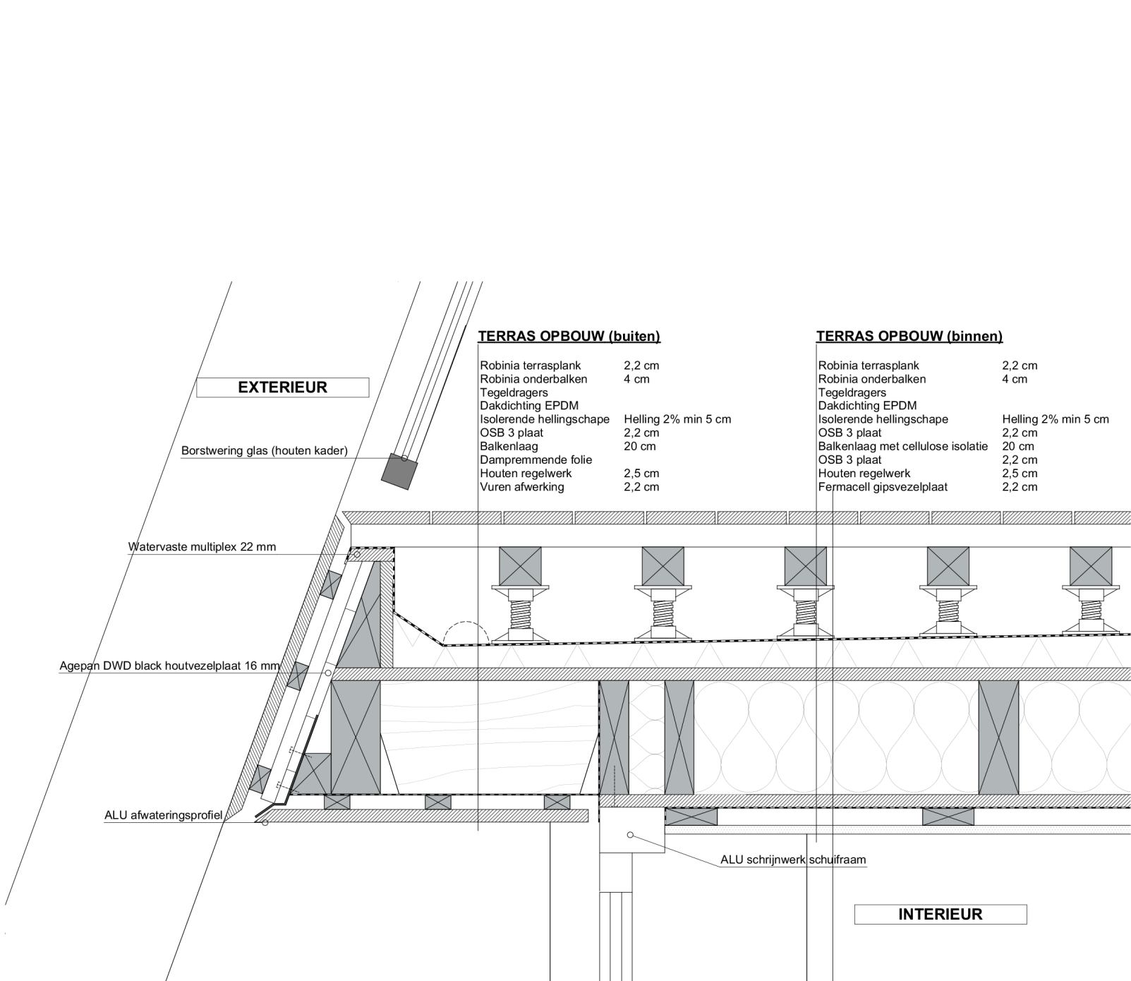
2D detail / archicad
