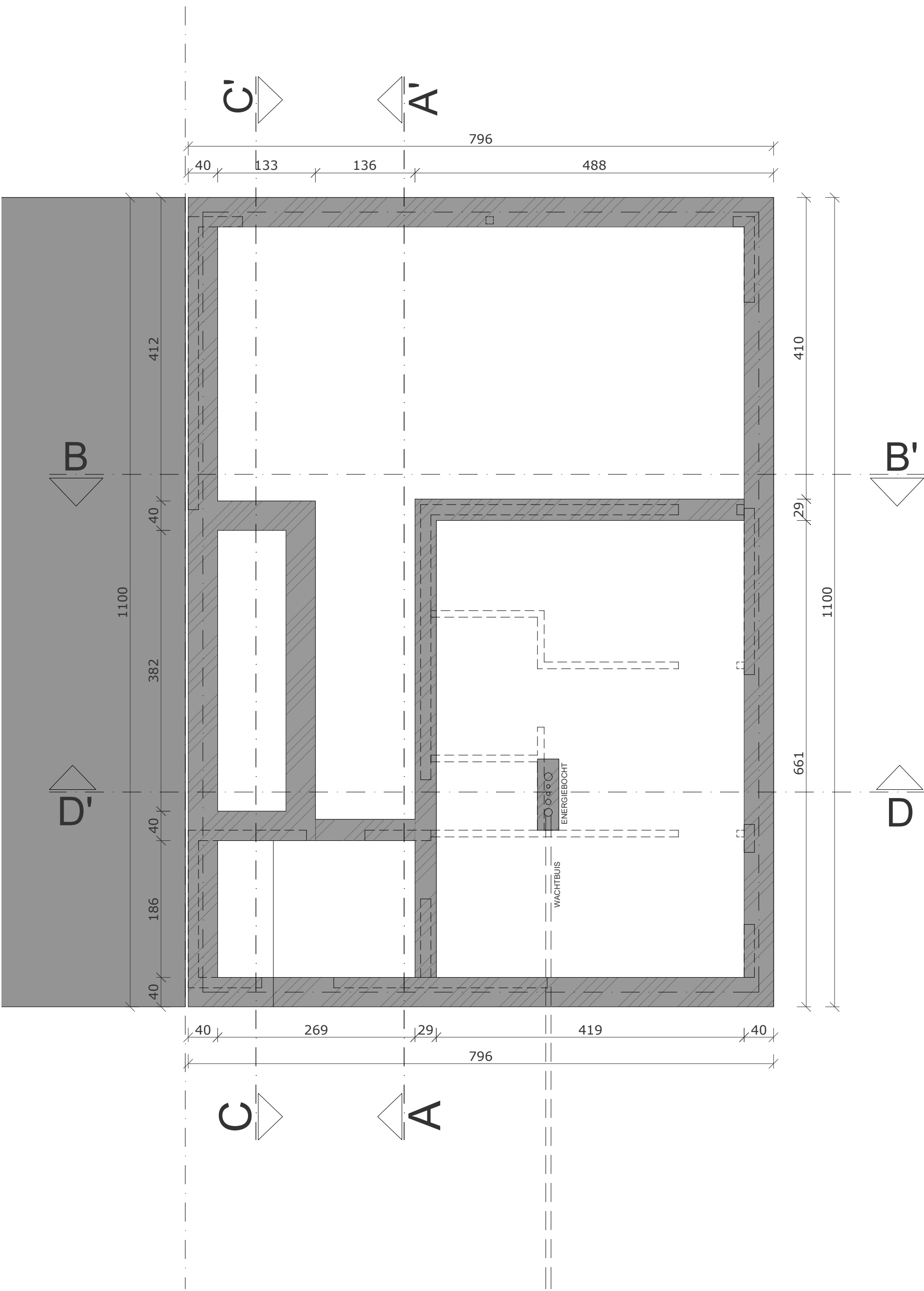
FUNDERINGSPLAN
